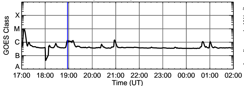
24-Mar-2011 (DOY 083) C1.3 @ 18:57:00 UT
