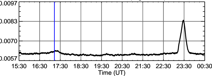
EVE Fe XVI 33.5 nm (log T=6.4)
