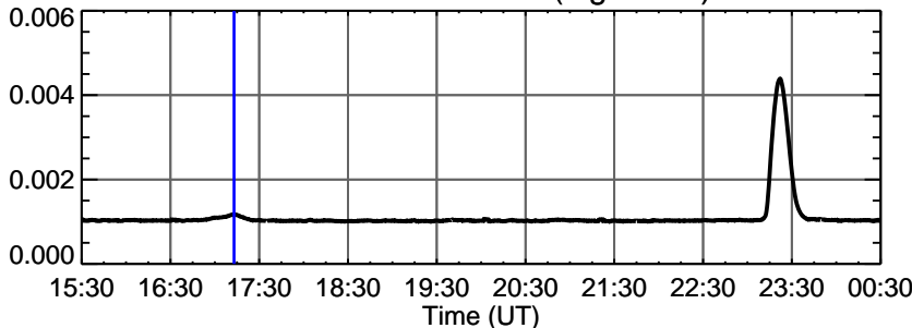
EVE Fe XVIII 9.4 nm (log T=6.8)
