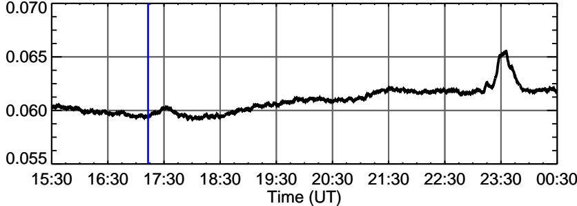
EVE Fe XV 28.4 nm (log T=6.3)
