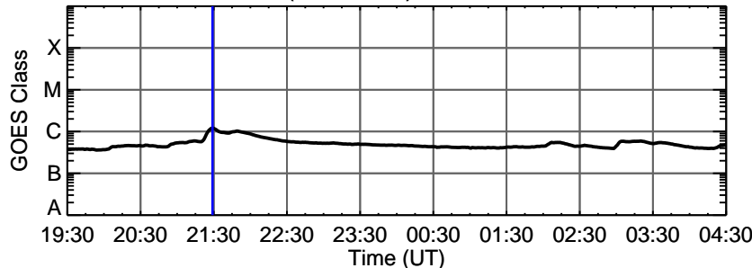
29-Mar-2011 (DOY 088) C1.2 @ 21:29:00 UT
