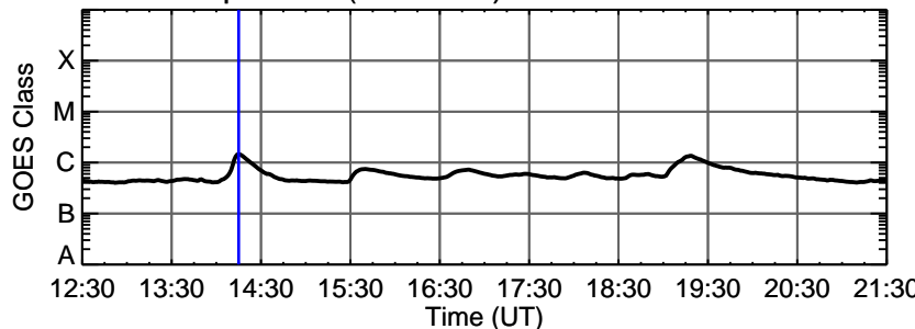
17-Apr-2011 (DOY 107) C1.4 @ 14:15:00 UT
