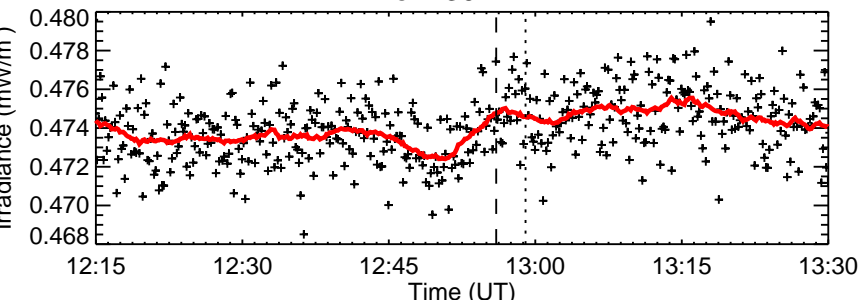
RHESHI Quicklook
