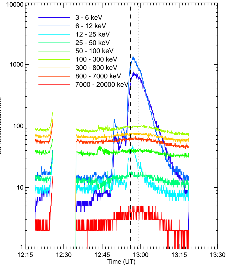
RHESHI Quicklook
