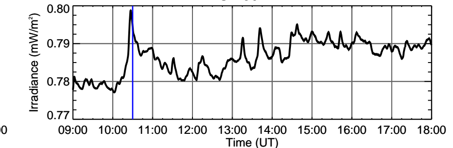
ESP 30.4 nm
