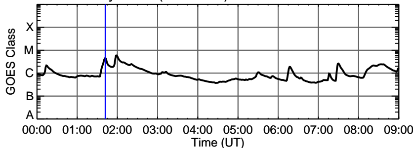
29-May-2011 (DOY 149) C4.6 @ 01:42:00 UT
