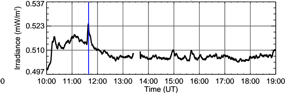
ESP 30.4 nm
