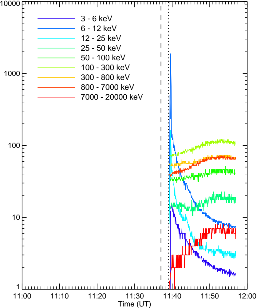
RHESSEI Quicklook
