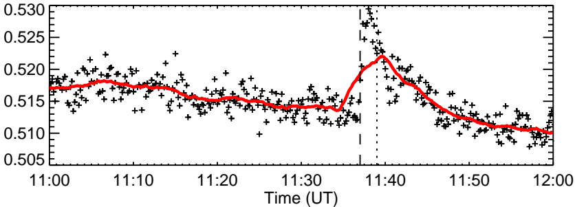
RHESSEI Quicklook
