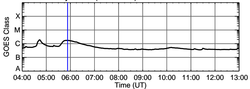
31-May-2011 (DOY 151) C1.7 @ 05:53:00 UT
