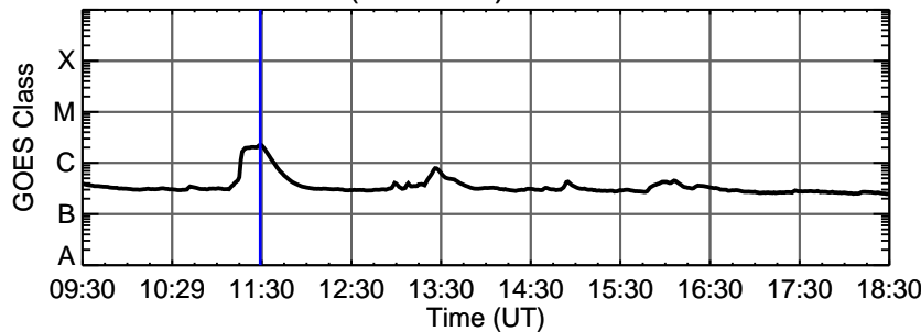
14-Jun-2011 (DOY 165) C2.2 @ 11:29:00 UT
