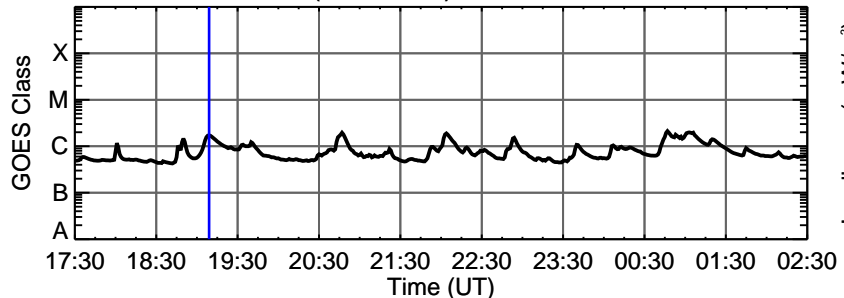
31-Jul-2011 (DOY 212) C1.7 @ 19:09:00 UT
