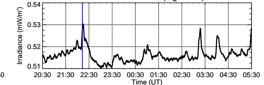
ESP 30.4 nm
