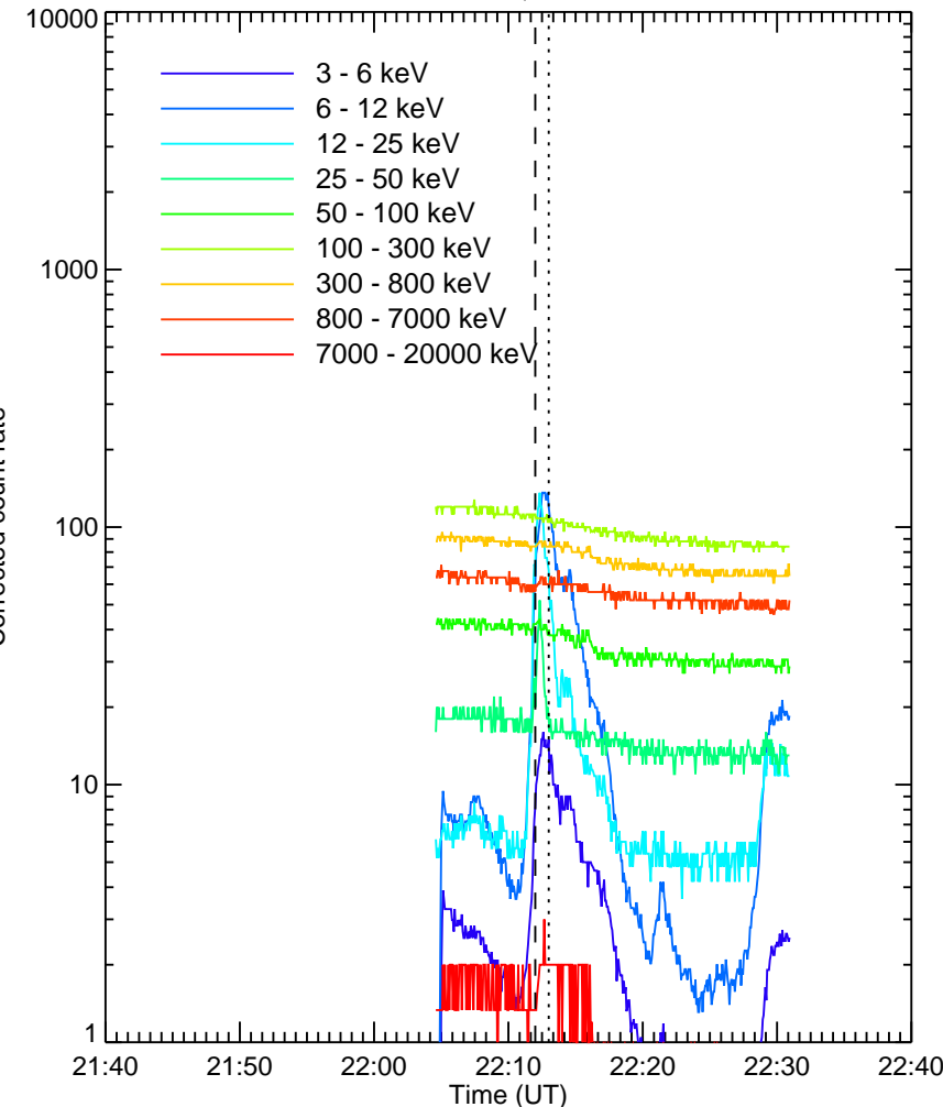
RHESSEI Quicklook
