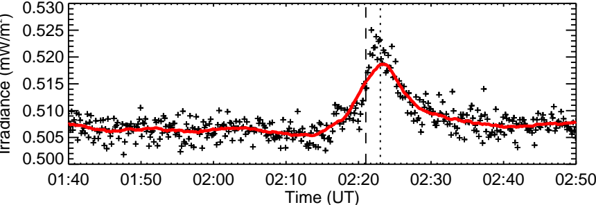
RHESSI Quicklook
