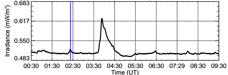
ESP 30.4 nm
