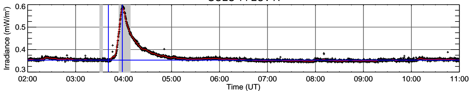
GOES-14 EUV-B
