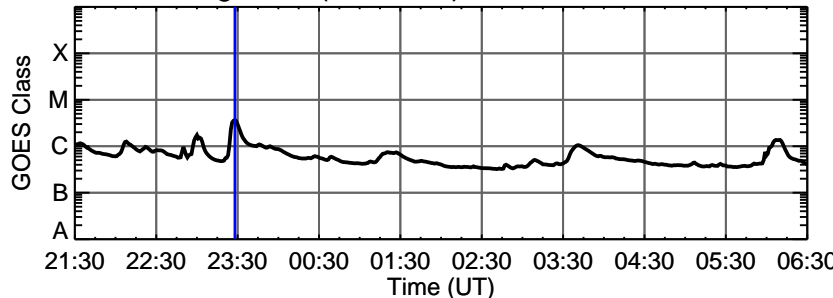
04-Aug-2011 (DOY 216) C3.6 @ 23:28:00 UT
