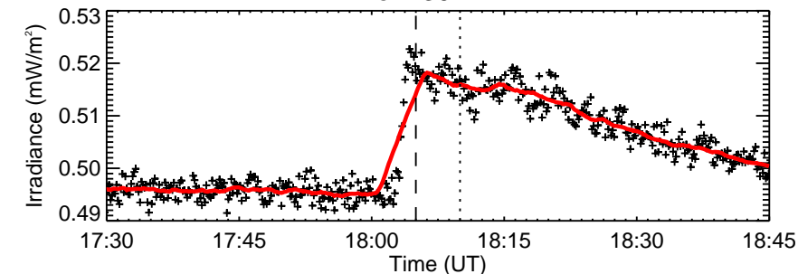
RHESHI Quicklook
