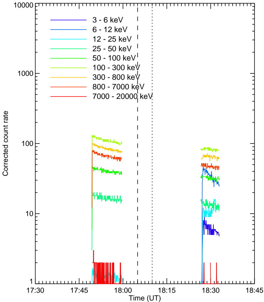
RHESHI Quicklook
