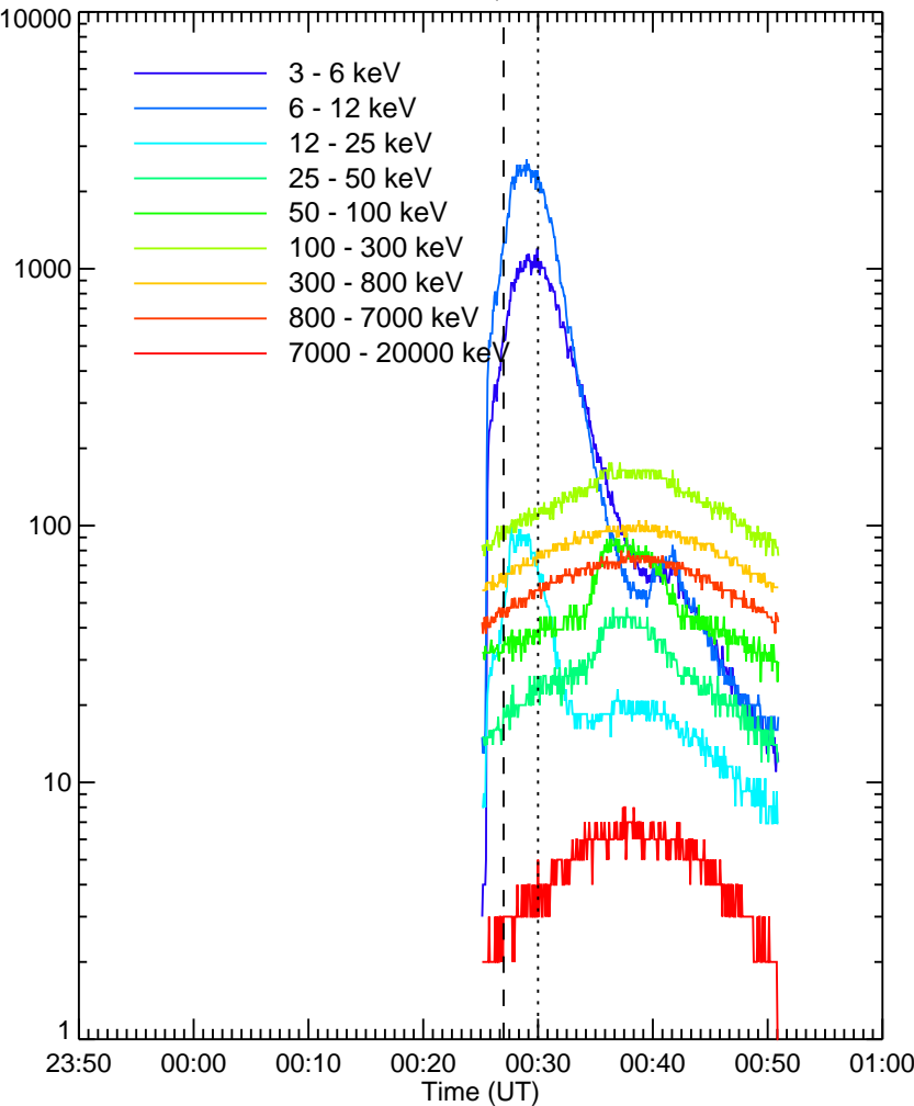
RHESSEI Quicklook
