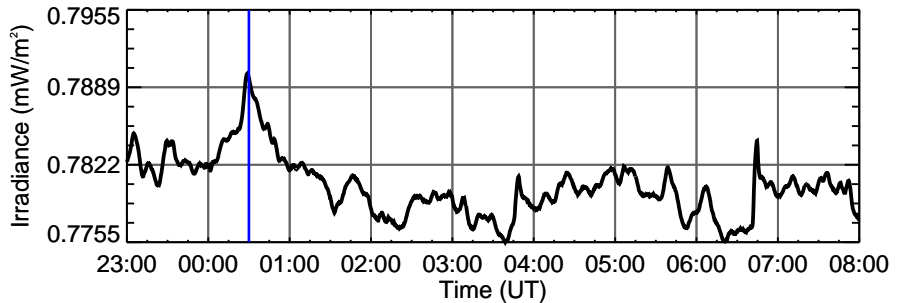
ESP 30.4 nm
