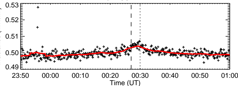
RHESSEI Quicklook
