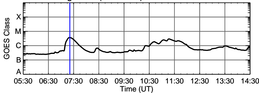
29-Aug-2011 (DOY 241) C3.7 @ 07:21:00 UT
