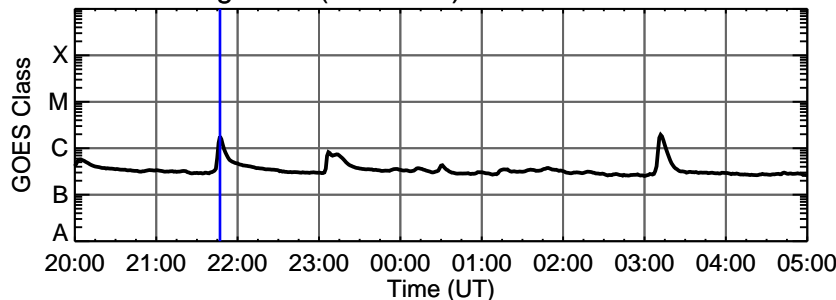
29-Aug-2011 (DOY 241) C1.7 @ 21:47:00 UT
