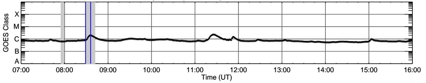
EVE Fe XX 13.3 nm (log T=7.0)
