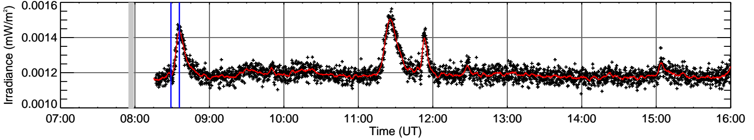
EVE Fe XVIII 9.4 nm (log T=6.8)
