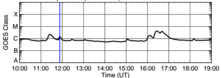
14-Sep-2011 (DOY 257) C1.4 @ 11:53:00 UT
