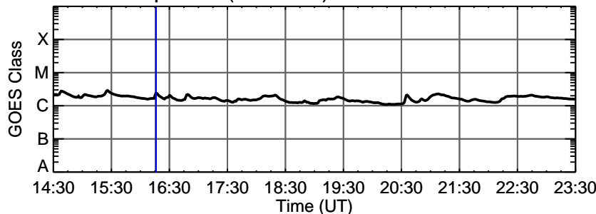
21-Sep-2011 (DOY 264) C2.3 @ 16:16:00 UT
