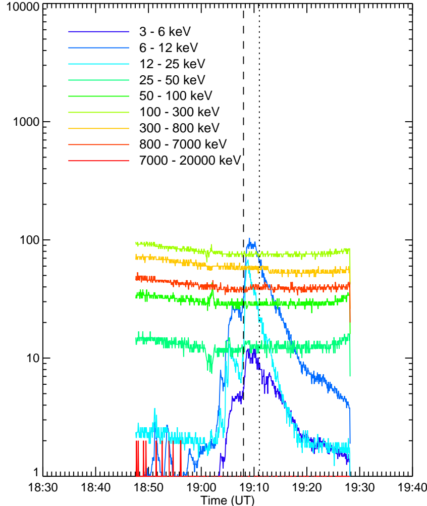
RHESSI Quicklook
