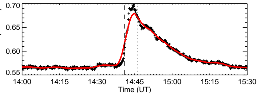
RHESSEI Quicklook
