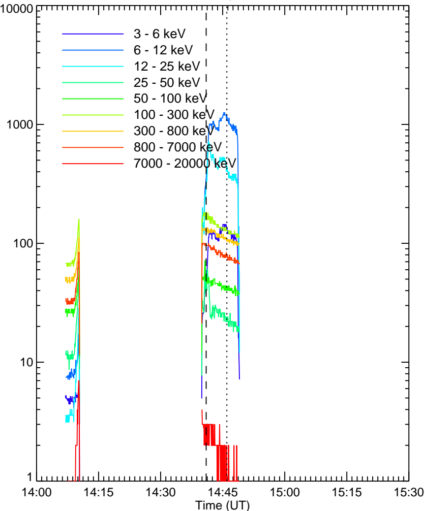
RHESSEI Quicklook
