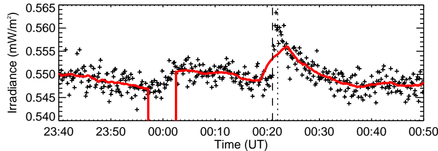
RHESSI Quicklook
