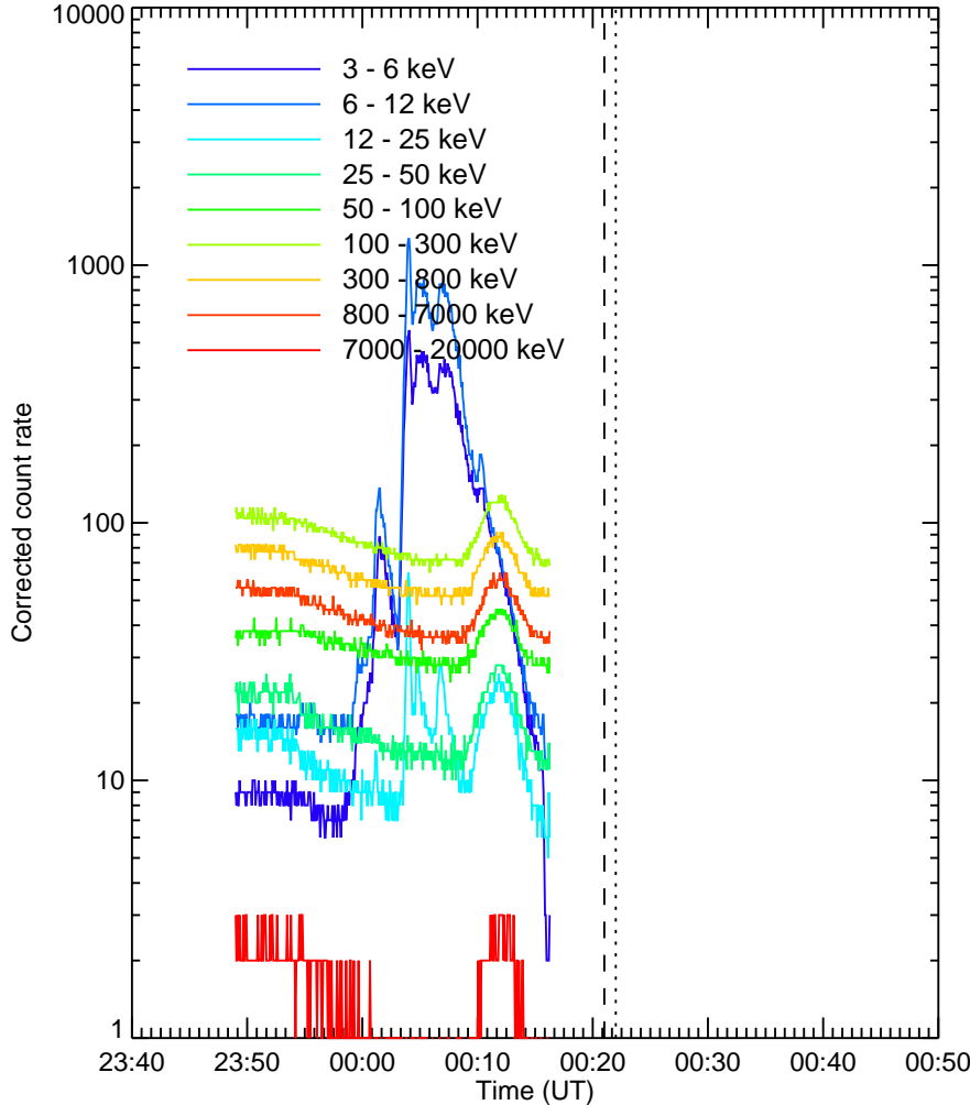
RHESSI Quicklook
