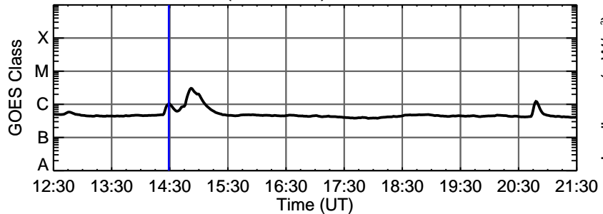
29-Oct-2011 (DOY 302) C1.0 @ 14:29:00 UT
