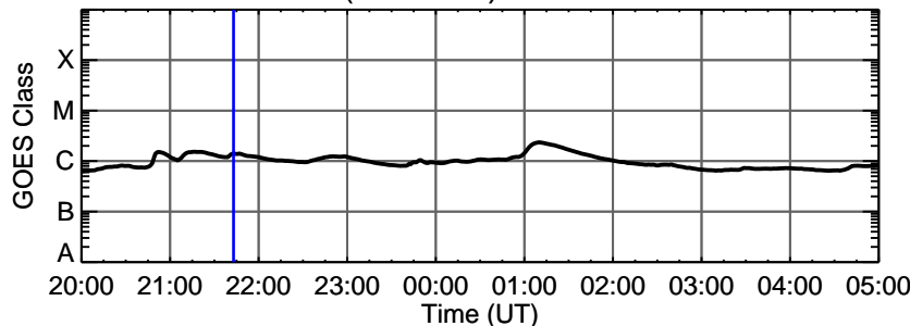
30-Oct-2011 (DOY 303) C1.4 @ 21:43:00 UT
