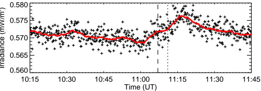
RHESSEI Quicklook
