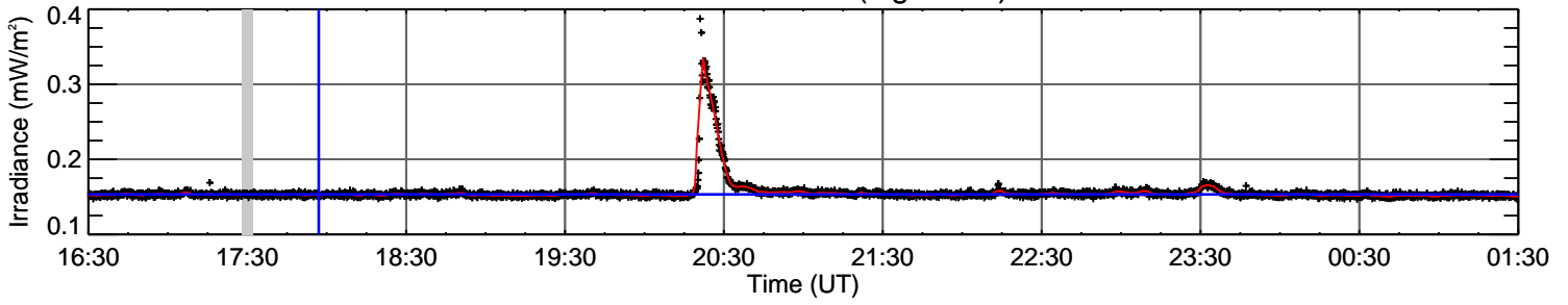
EVE He II 25.6 nm (log T=4.8)
