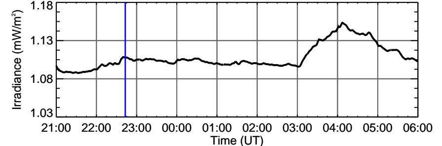
ESP 30.4 nm
