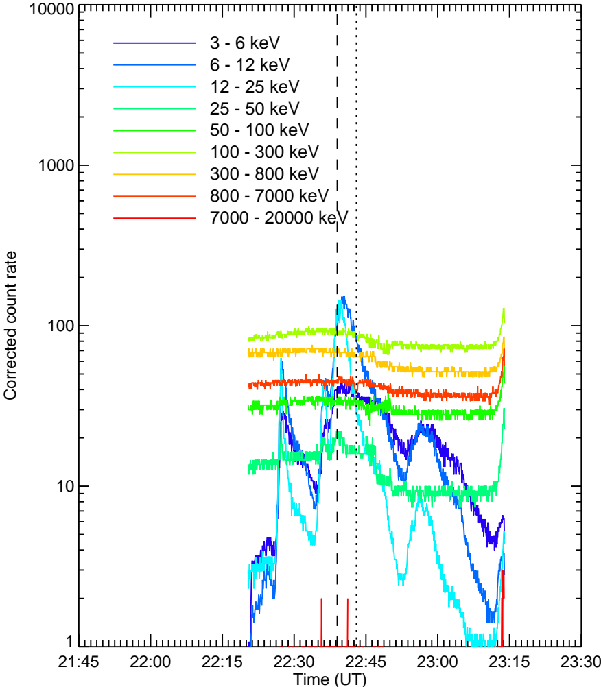
RHESSI Quicklook
