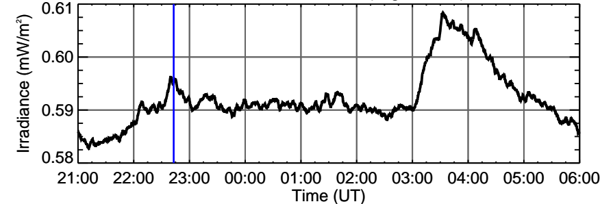
ESP 30.4 nm
