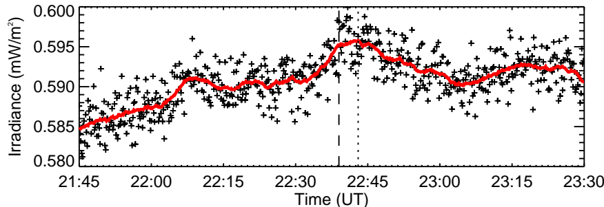
RHESSI Quicklook
