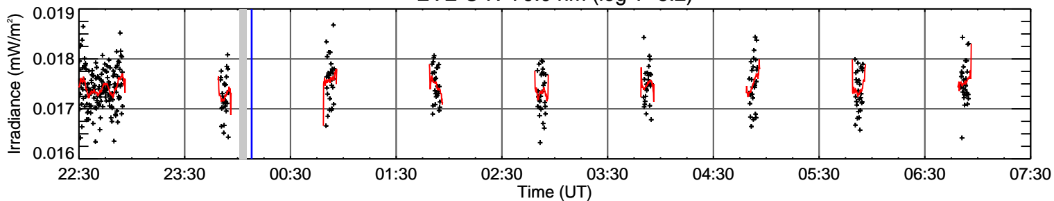
EVE O IV 55.4 nm (log T=5.2)
