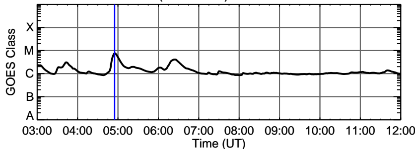
16-Nov-2011 (DOY 320) C7.5 @ 04:55:00 UT
