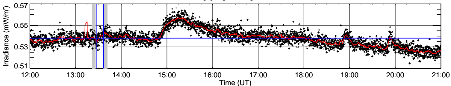
GOES-14 EUV-B
