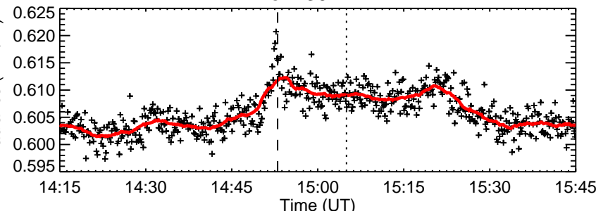
RHESSI Quicklook
