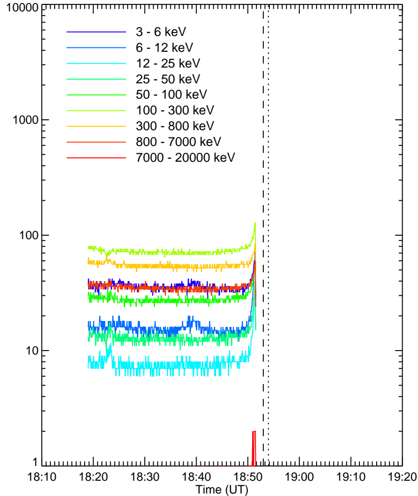
RHESSI Quicklook
