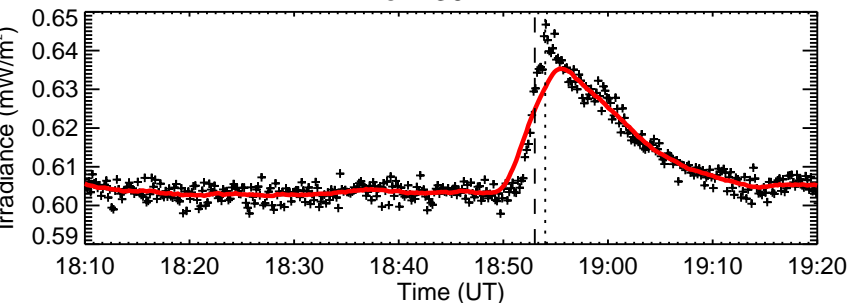
RHESSI Quicklook
