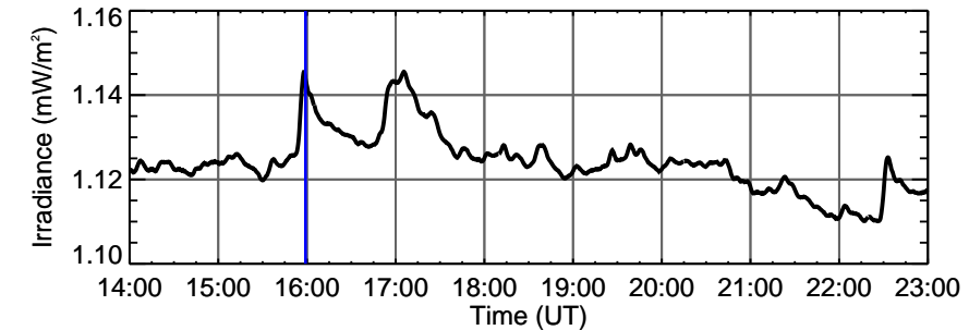
ESP 30.4 nm
