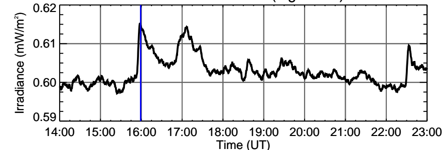
ESP 30.4 nm
