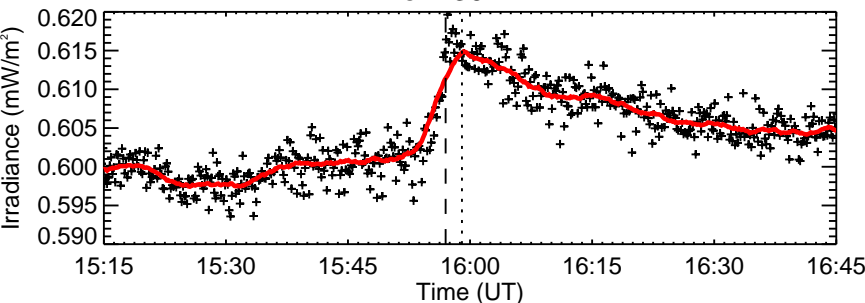
RHESSI Quicklook
