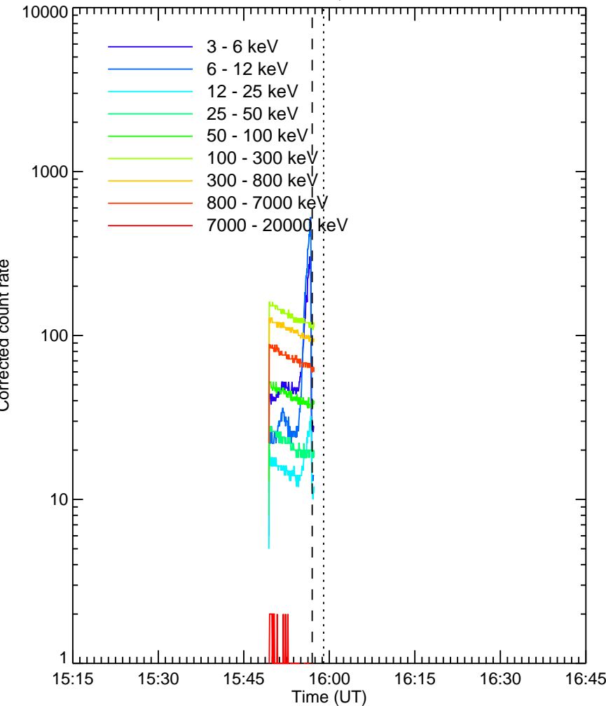
RHESSI Quicklook
