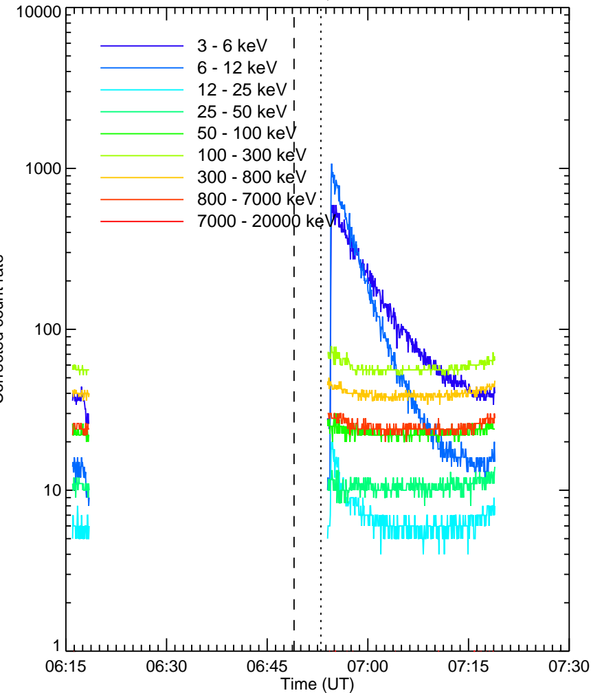
RHESSI Quicklook
