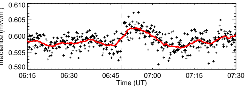
RHESSI Quicklook
