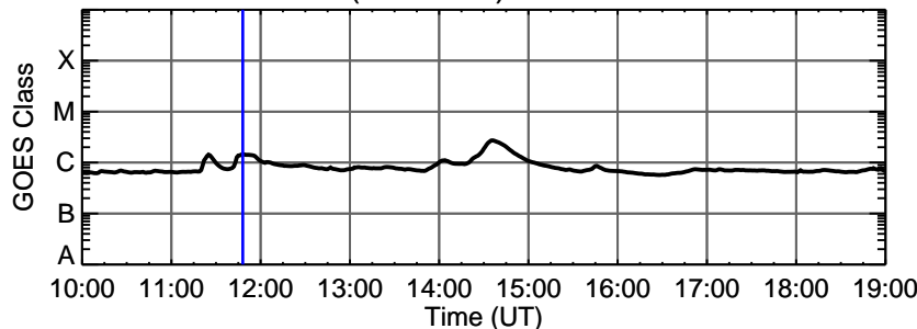
19-Nov-2011 (DOY 323) C1.4 @ 11:48:00 UT
