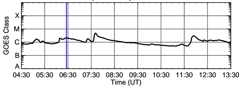
20-Nov-2011 (DOY 324) C2.1 @ 06:26:00 UT
