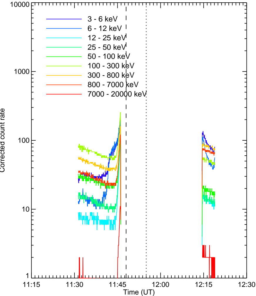
RHESSI Quicklook
