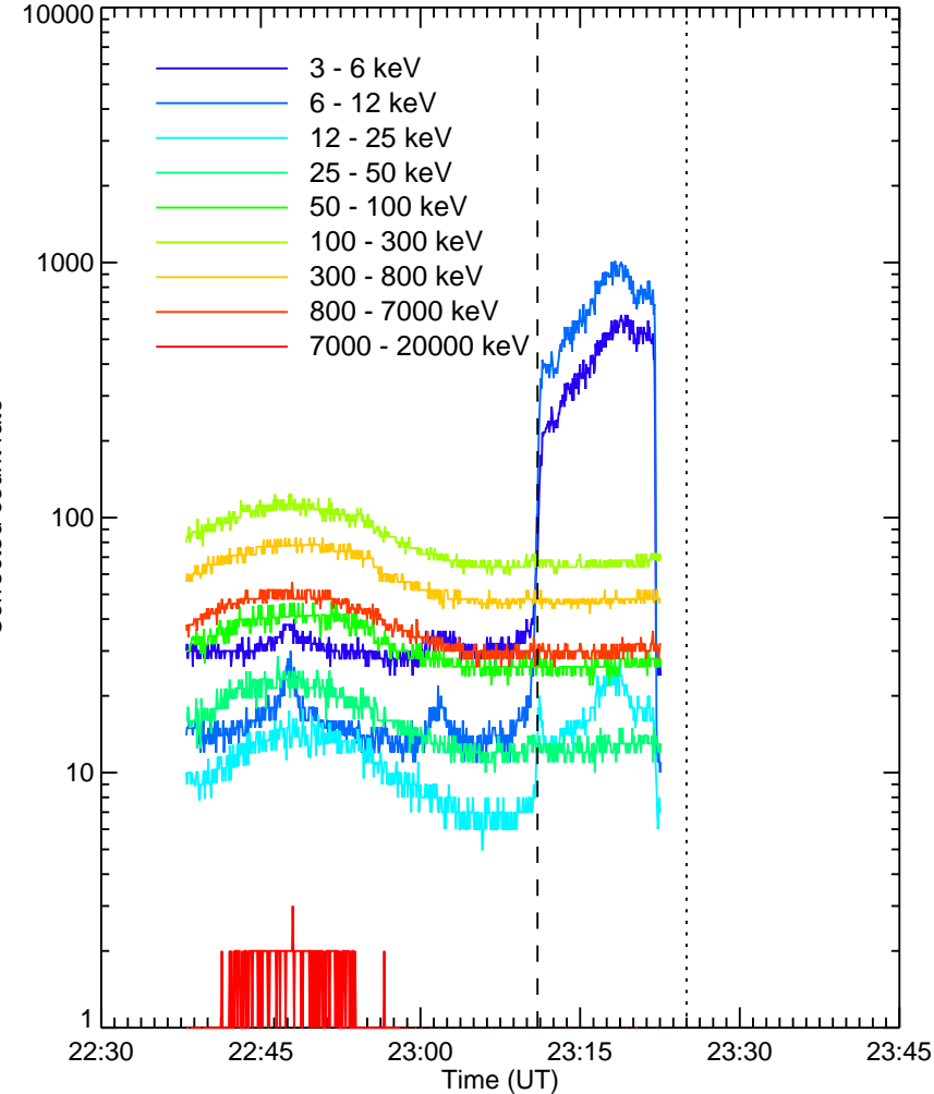
RHESHI Quicklook
