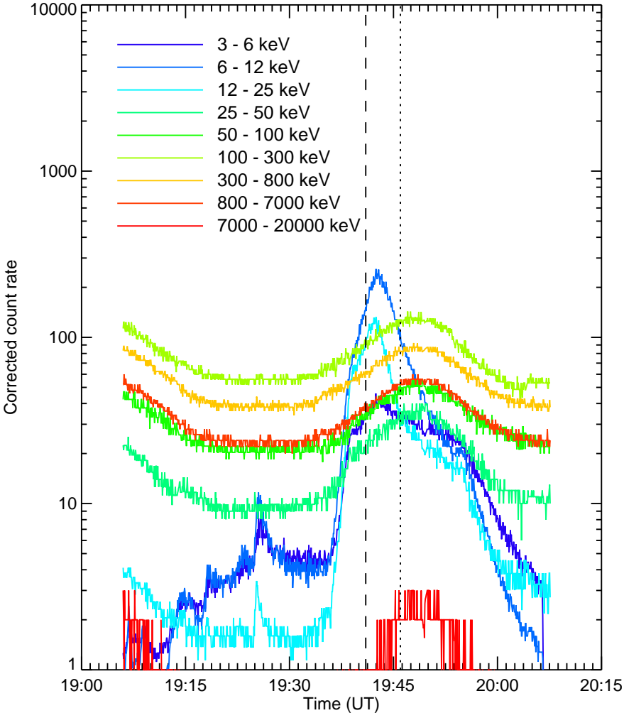
RHESSEI Quicklook
