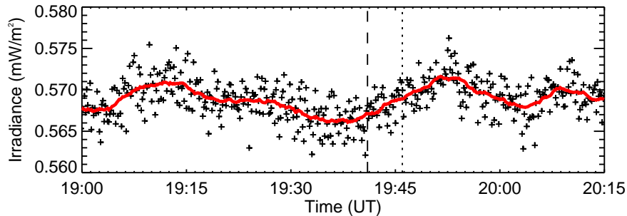
RHESSEI Quicklook
