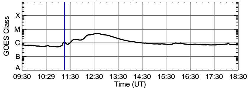
24-Dec-2011 (DOY 358) C1.1 @ 11:16:00 UT
