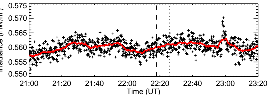
RHESSEI Quicklook
