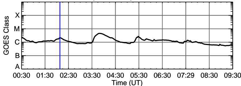
28-Dec-2011 (DOY 362) C2.1 @ 02:08:00 UT
