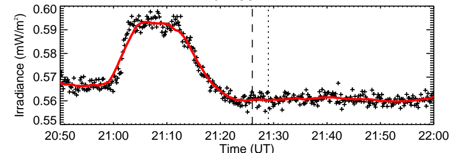
RHESSI Quicklook
