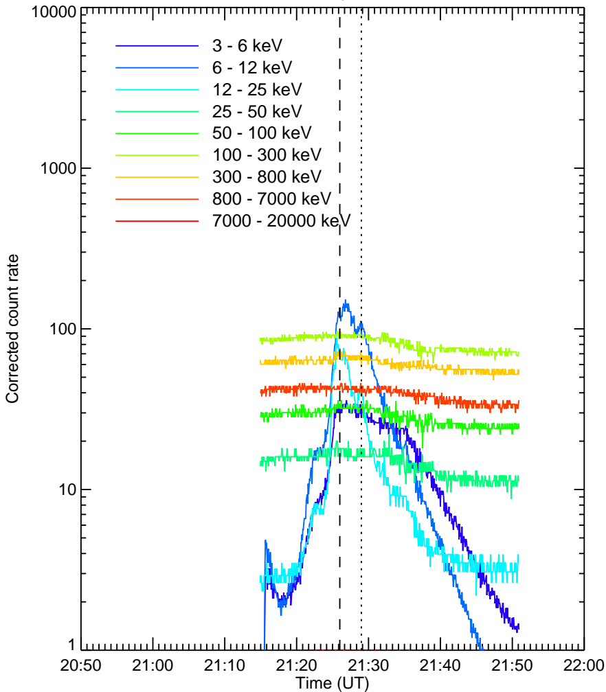
RHESSI Quicklook
