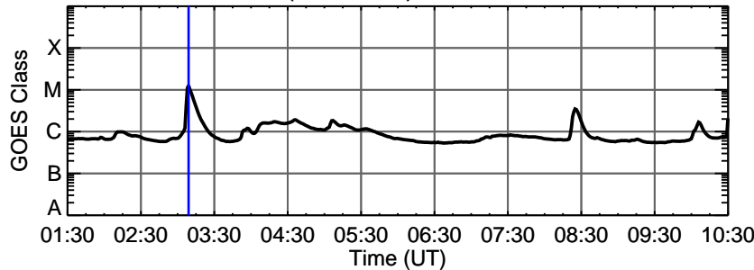
30-Dec-2011 (DOY 364) M1.2 @ 03:09:00 UT
