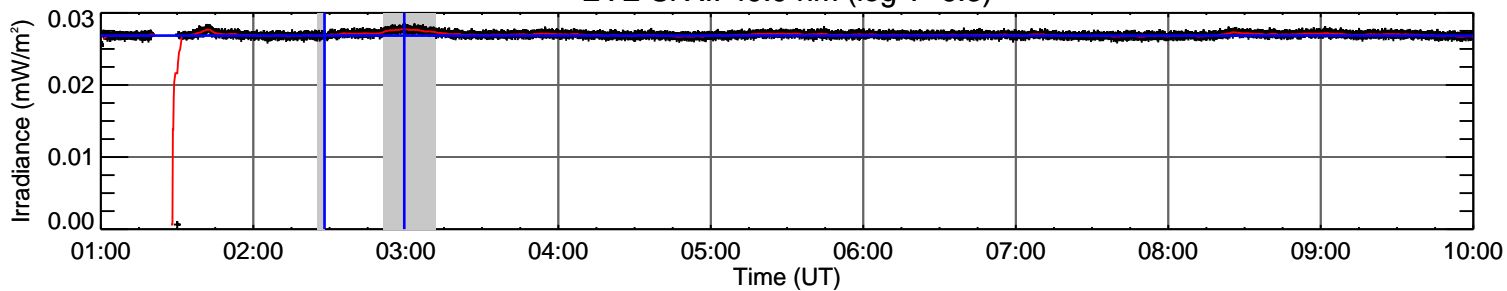
EVE Fe XIV 21.1 nm (log T=6.3)
