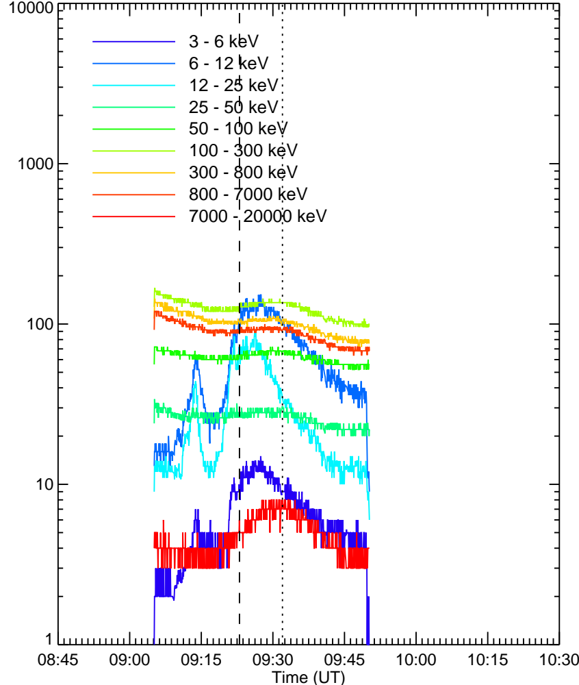
RHESSI Quicklook
