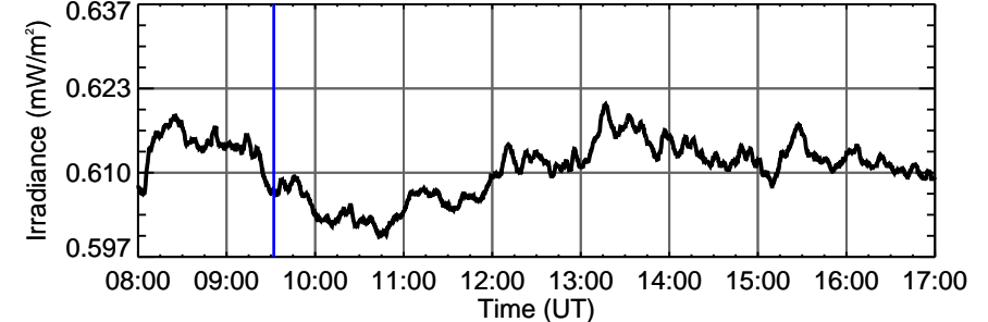
ESP 30.4 nm
