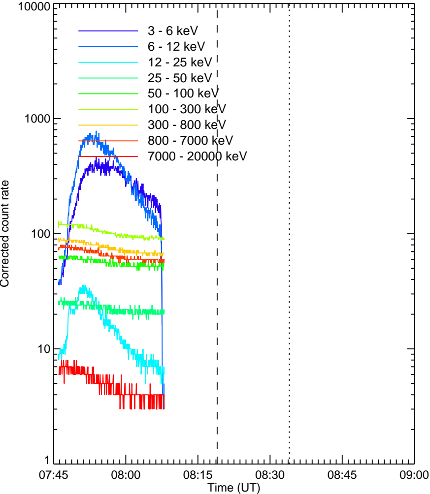
RHESSE Quicklook
