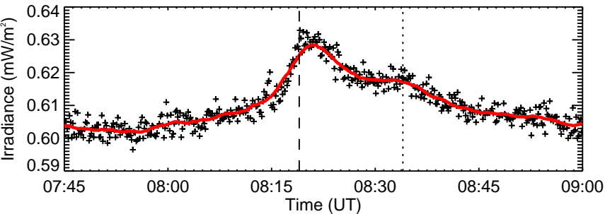
RHESSE Quicklook
